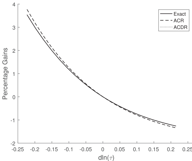
FIGURE 2 Welfare gains relative to baseline ( \tau = 1.56 ), Pareto
