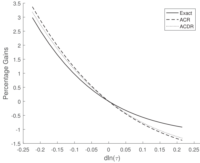
FIGURE 3 Welfare gains relative to baseline ( \tau = 1.66 ), log-normal
